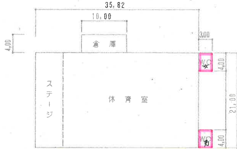
⑩ 1F
